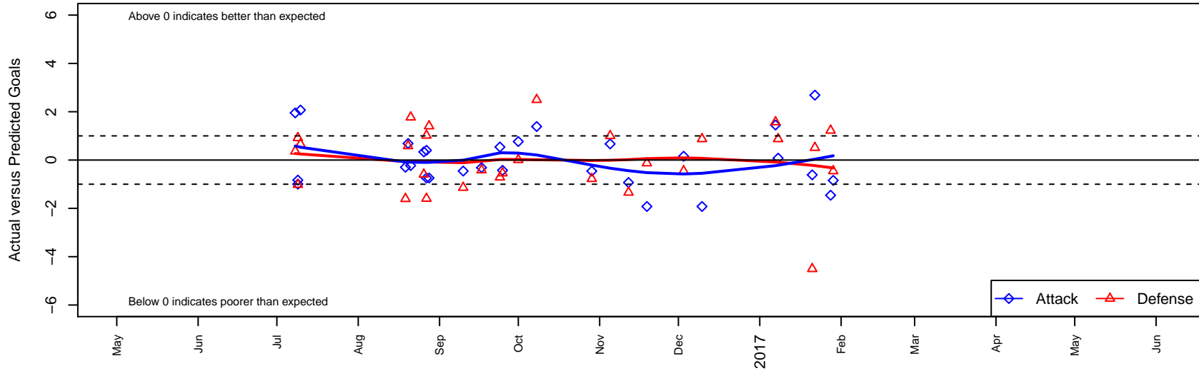
Seattle United W Blue B03 Dots are actual minus expected GF (blue circles) and GA (red triangles). Blue line is smoothed change in attack strength. Red is smoothed change in defense strength.
